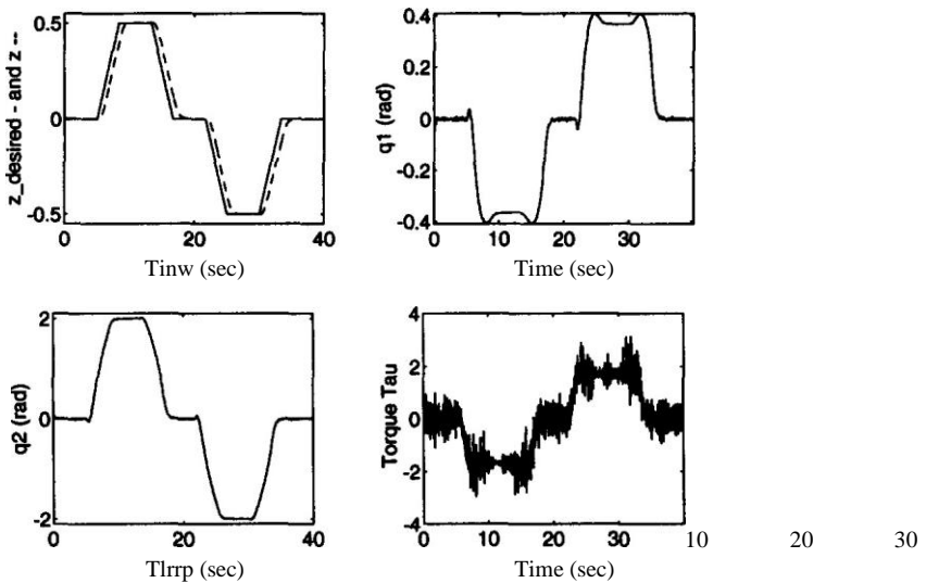
Figure 19. Visual servo of the acrobot with no distortions (see text).
