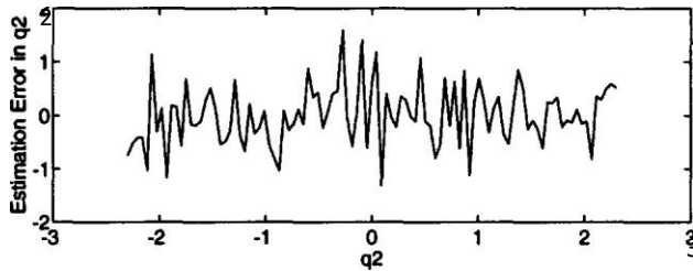
Figure 12. Error in visual state estimation with no distortions.
