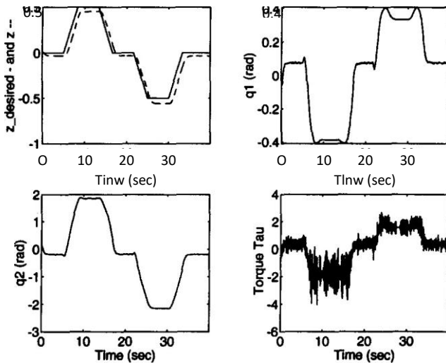
Figure 23. Visual servo with PI = 0.015 (see text).
