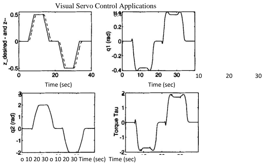
Figure 20. Rolling acrobot under full state feedback control (see text).
