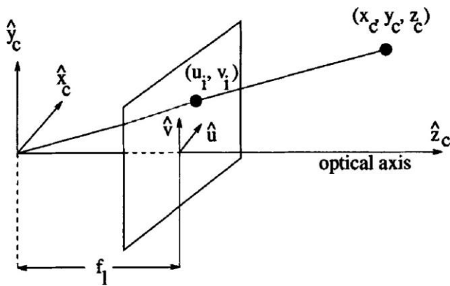
Figure 3. Pinhole lens with associated coordinate systems.
