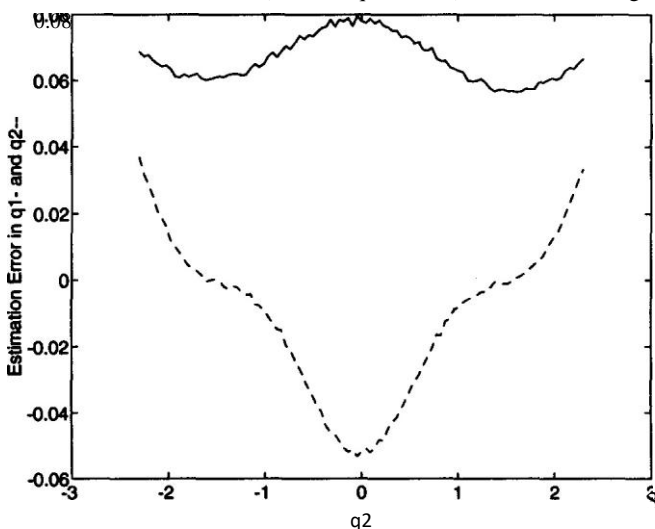
Figure 16. State estimation error (m solid, q2 dashed) under thin prism distortion ( s_1 = 0.1 ).
