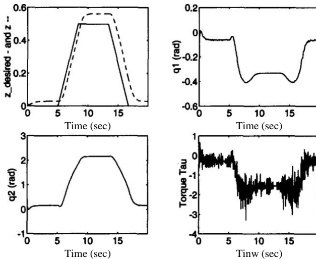
Figure 25. Visual servo with p_a = 0.015 (see text).
