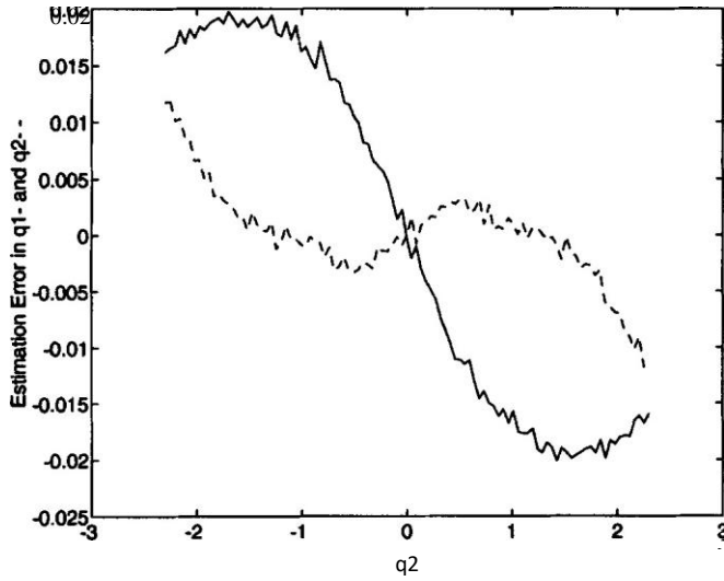
Figure 13. State —timation error (m solid, q'z dashed) under radial distortion ( k_1 = 0.1 ).
