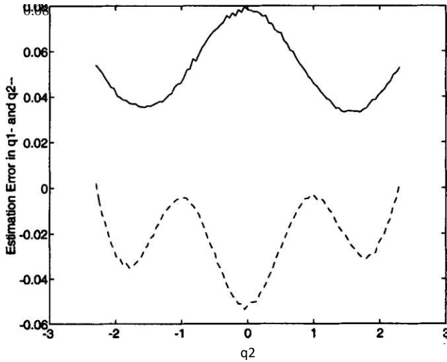
Figure 14. State —timation error (m solid, q'2 dashed) under decentering distortion ( PI = 0.1 ).
