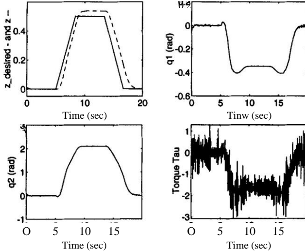
Figure 27. Visual servo with s_2 = 0.025 (see text).
