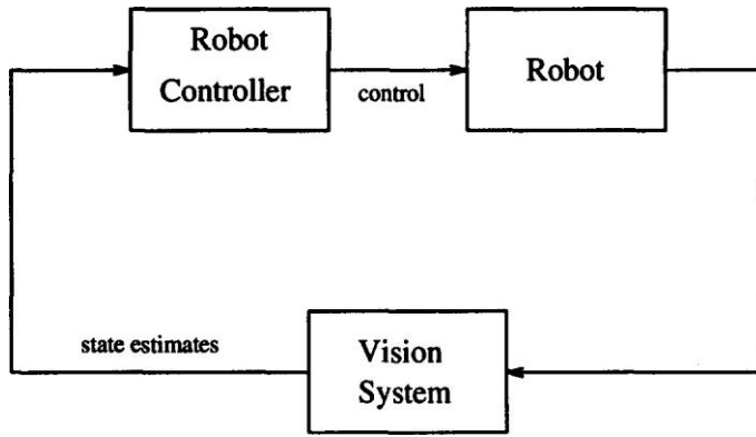
Figure 2. Direct visual servo.
