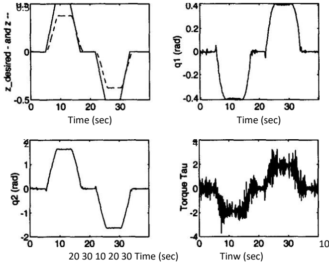
Figure 21. Visual servo with k_l = 0.1 (see text).
