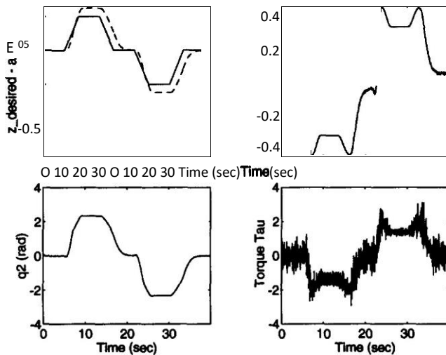
Figure 22. Visual servo with k_l = -0.1 (see text).
