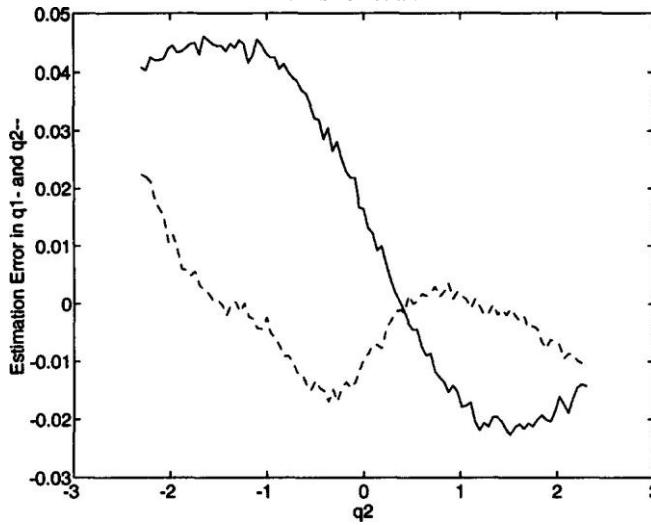
Figure 18. State atimation error (QI solid, dashed) under all aberrations.
