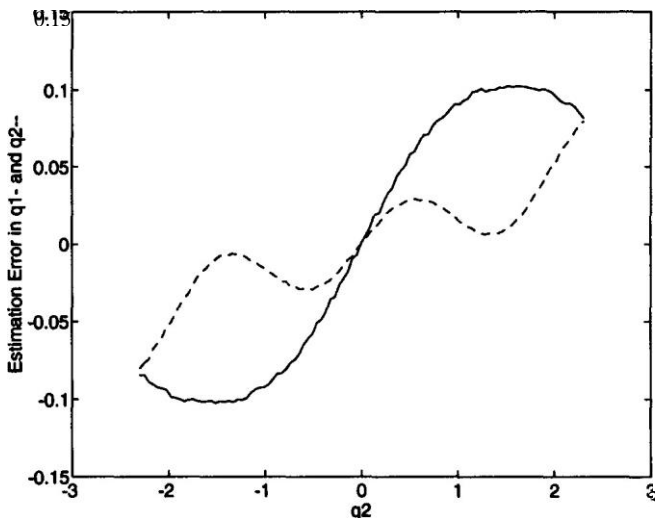
Figure 15. State estimation error (m solid, q1a dashed) under decentering distortion
