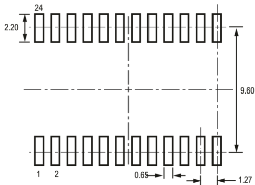
A PCB Layout Reference View
