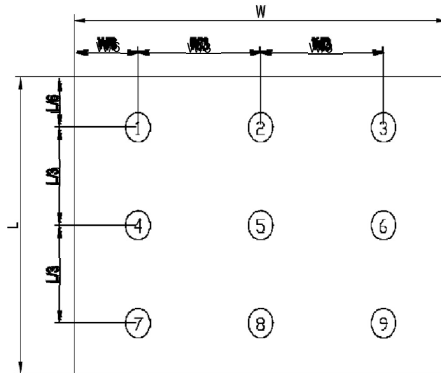
Measurement equipment PR-705 ( \Phi 8\text{mm} )
