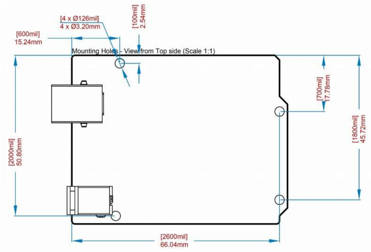
Board outline
