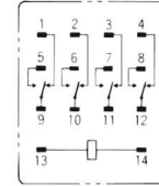
Terminal Arrangement/ Internal Connections (Bottom View)
