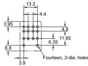
PCB Processing Dimensions (Bottom View)
