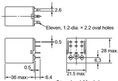
Standard Models
